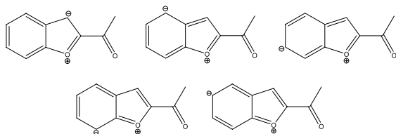
Figure 1. Resonance structures of 2-acetylbenzofuran representing the loci for further electrophilic substitution.
